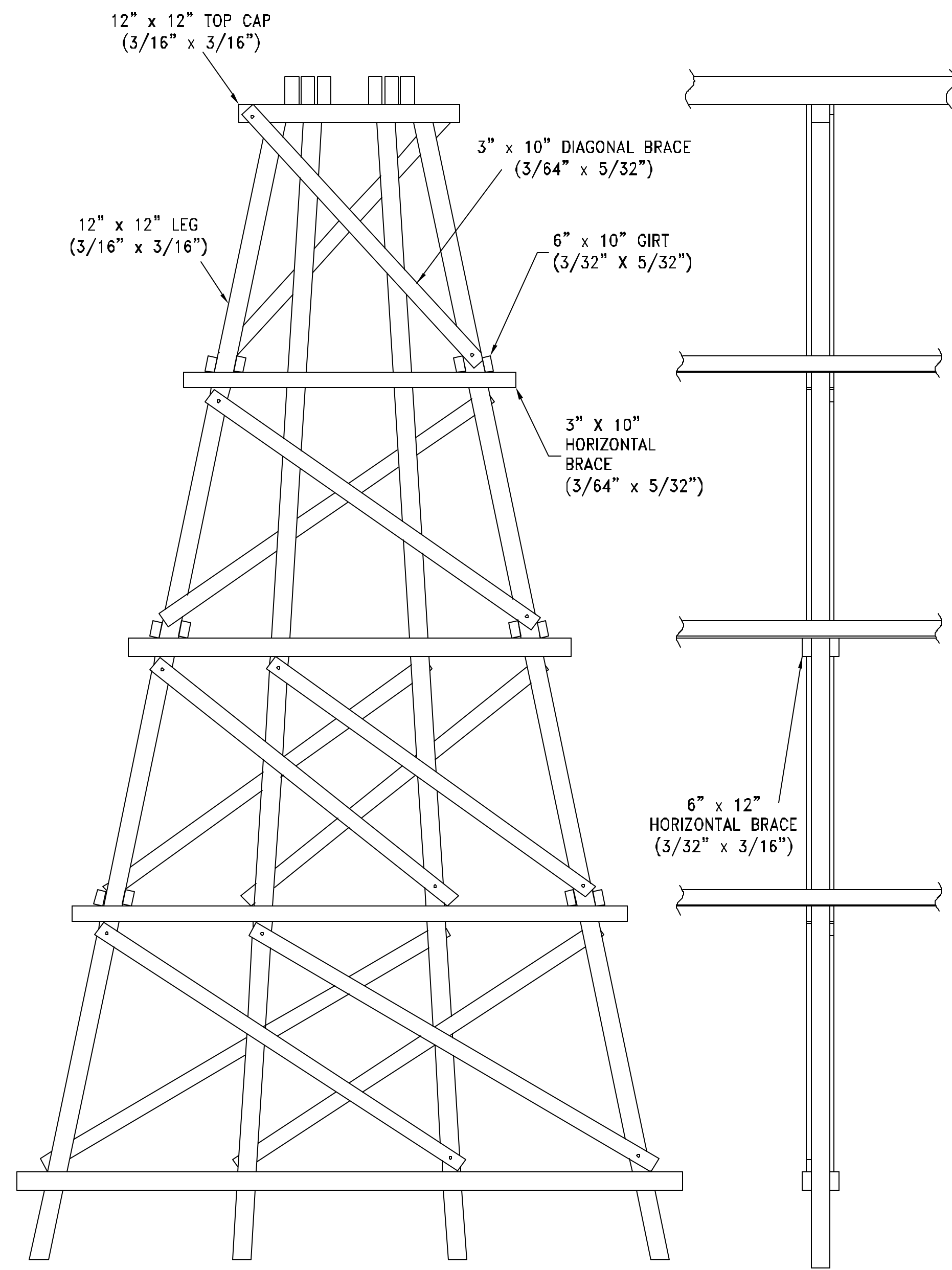
FALSE FRAME TRESTLE BENT
