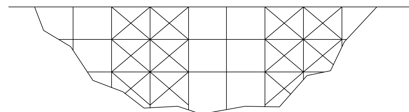
TYPICAL BRACING PATTERN
