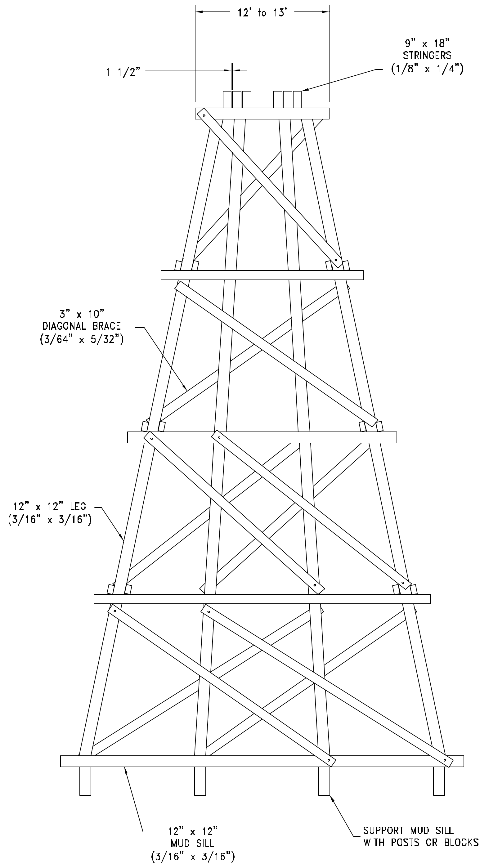
TRUE FRAME BENT or NOTCHED FRAME BENT
