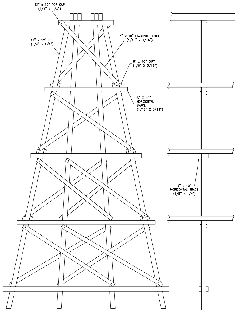
FALSE FRAME TRESTLE BENT
