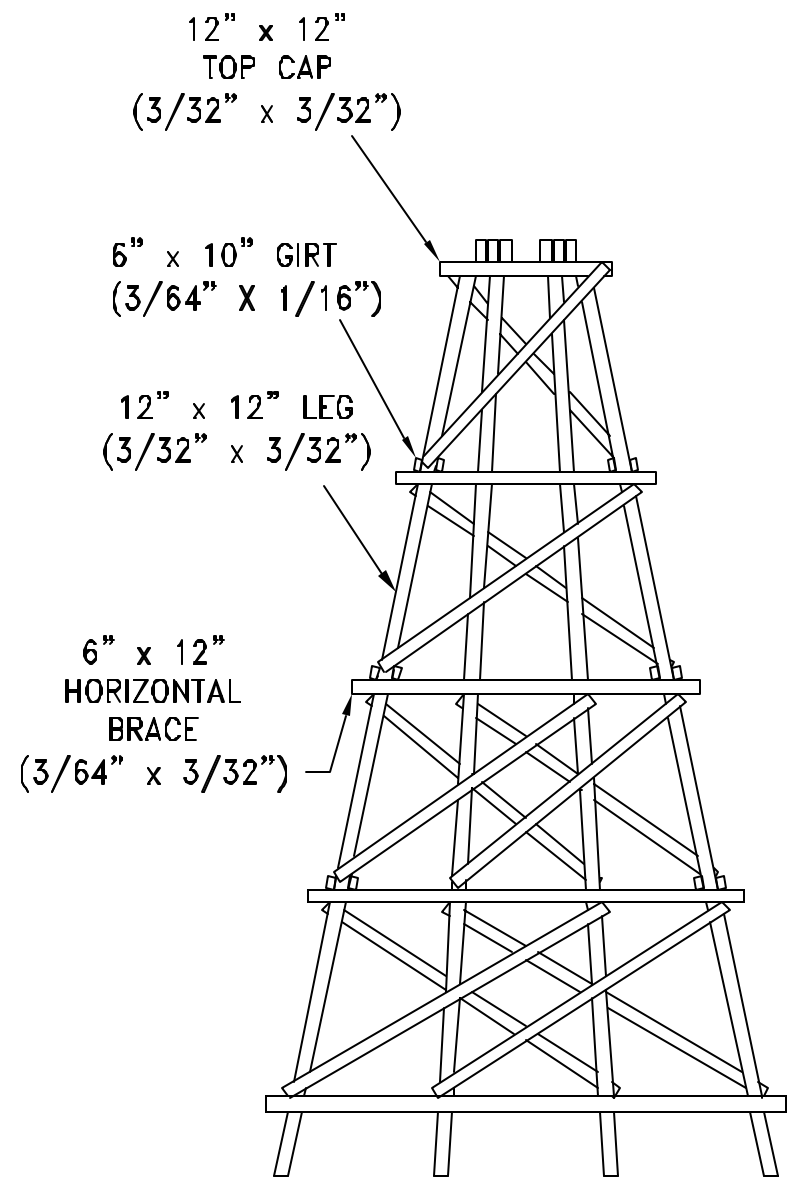
FALSE FRAME TRESTLE BENT
