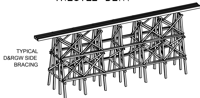
FALSE FRAME TRESTLE BENT
