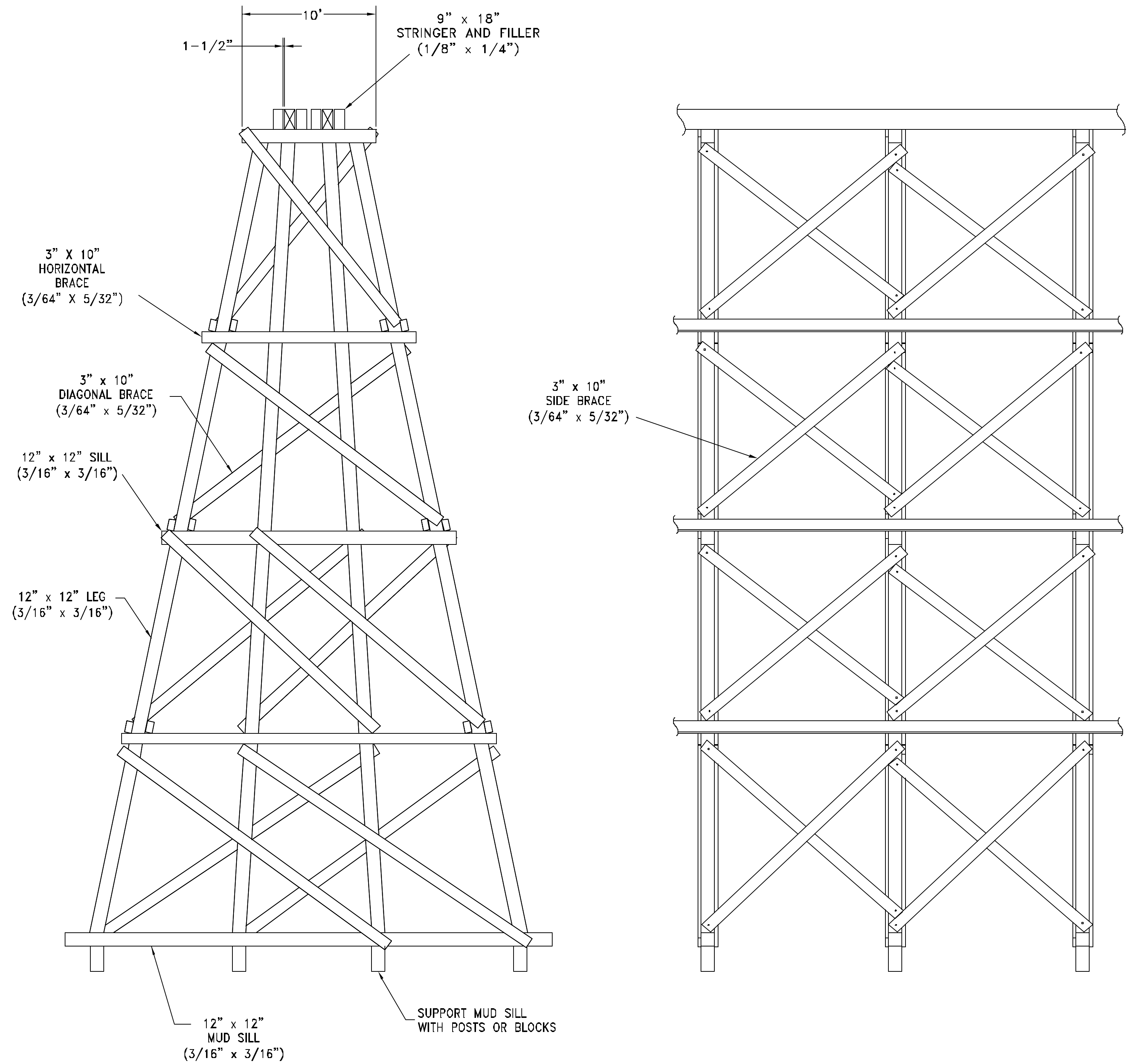
TRUE FRAME BENT or NOTCHED FRAME BENT
