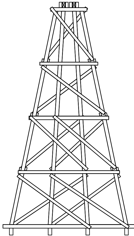
1 : 1 Drawing True or Notched Frame TJ4DNN Trestle Bent
