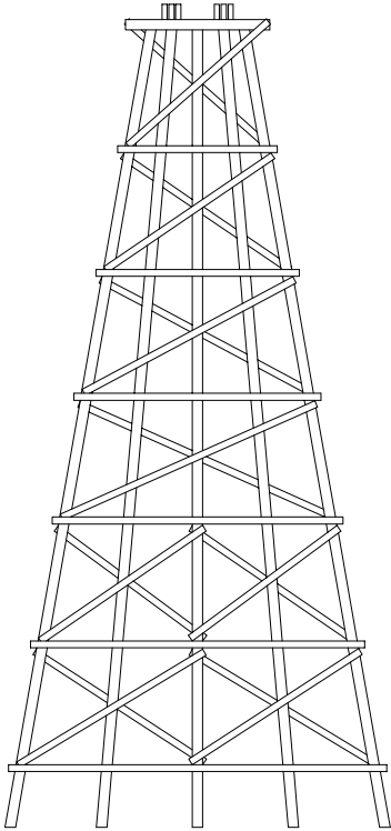
80' STANDARD GAUGE TRESTLE BENT FULL SIZE - N SCALE
