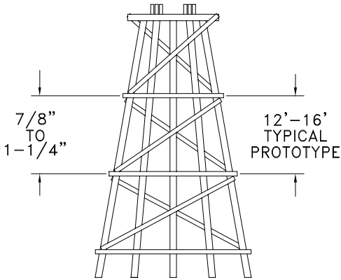
40' STANDARD GAUGE TRESTLE BENT FULL SIZE - N SCALE
