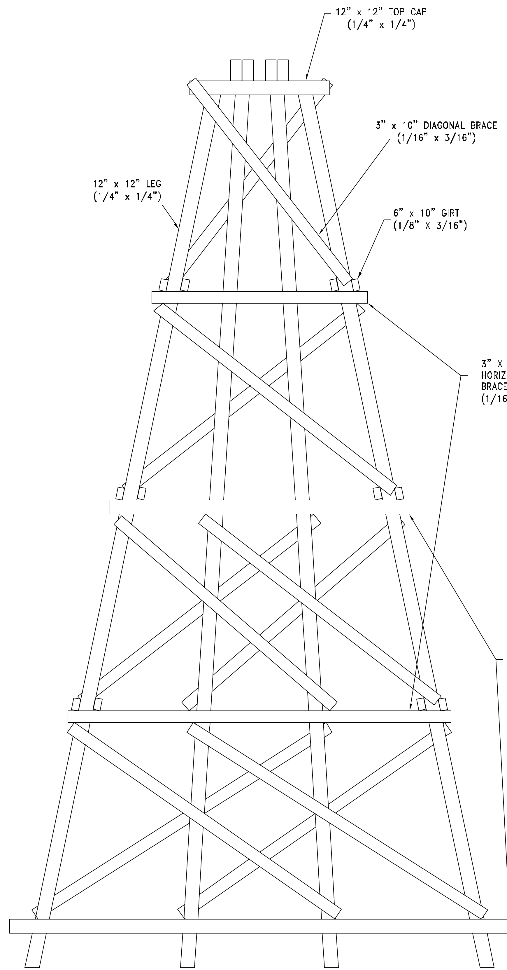
FALSE FRAME TRESTLE BENT
