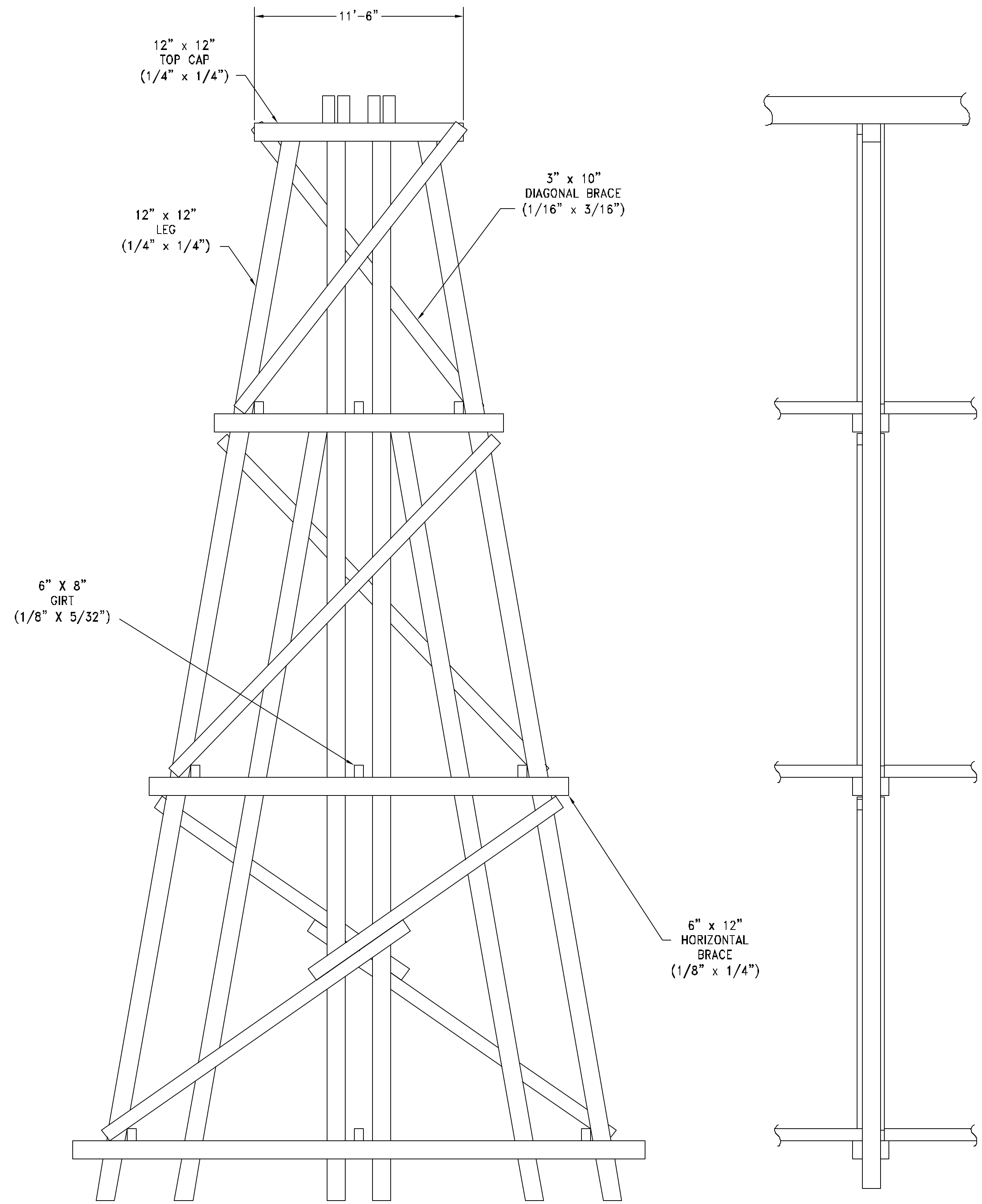
FALSE FRAME TRESTLE BENT
