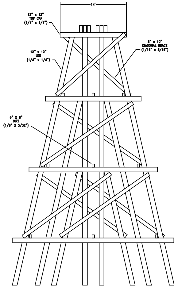
FALSE FRAME TRESTLE BENT
