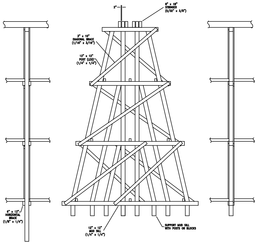
TRUE FRAME BENT or NOTCHED FRAME BENT
