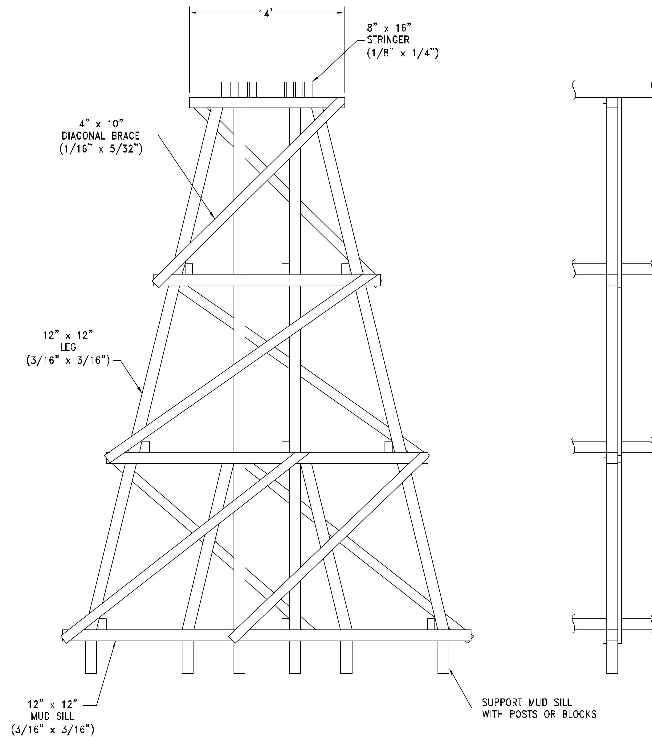
TRUE FRAME BENT or NOTCHED FRAME BENT
