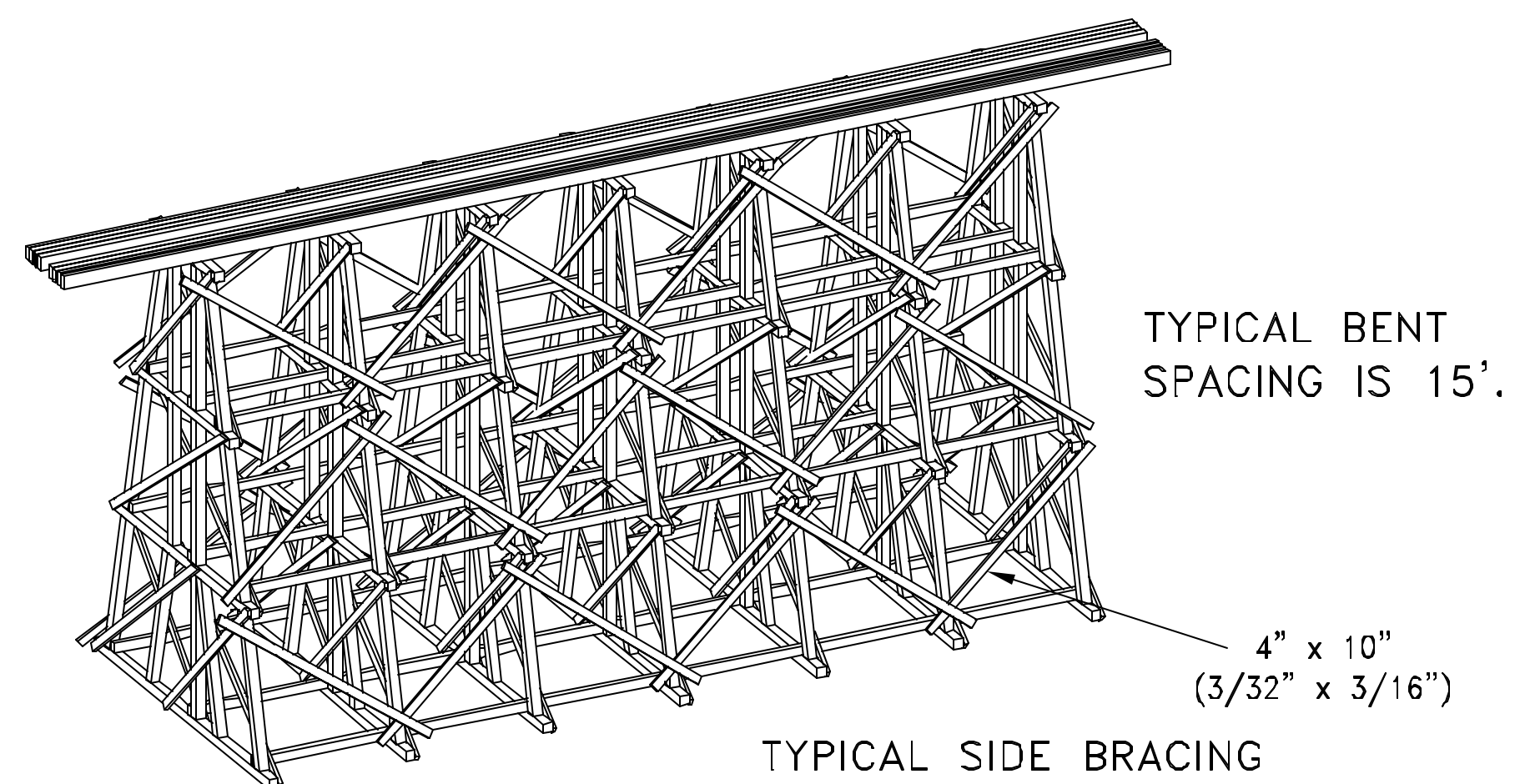
FALSE FRAME TRESTLE BENT
