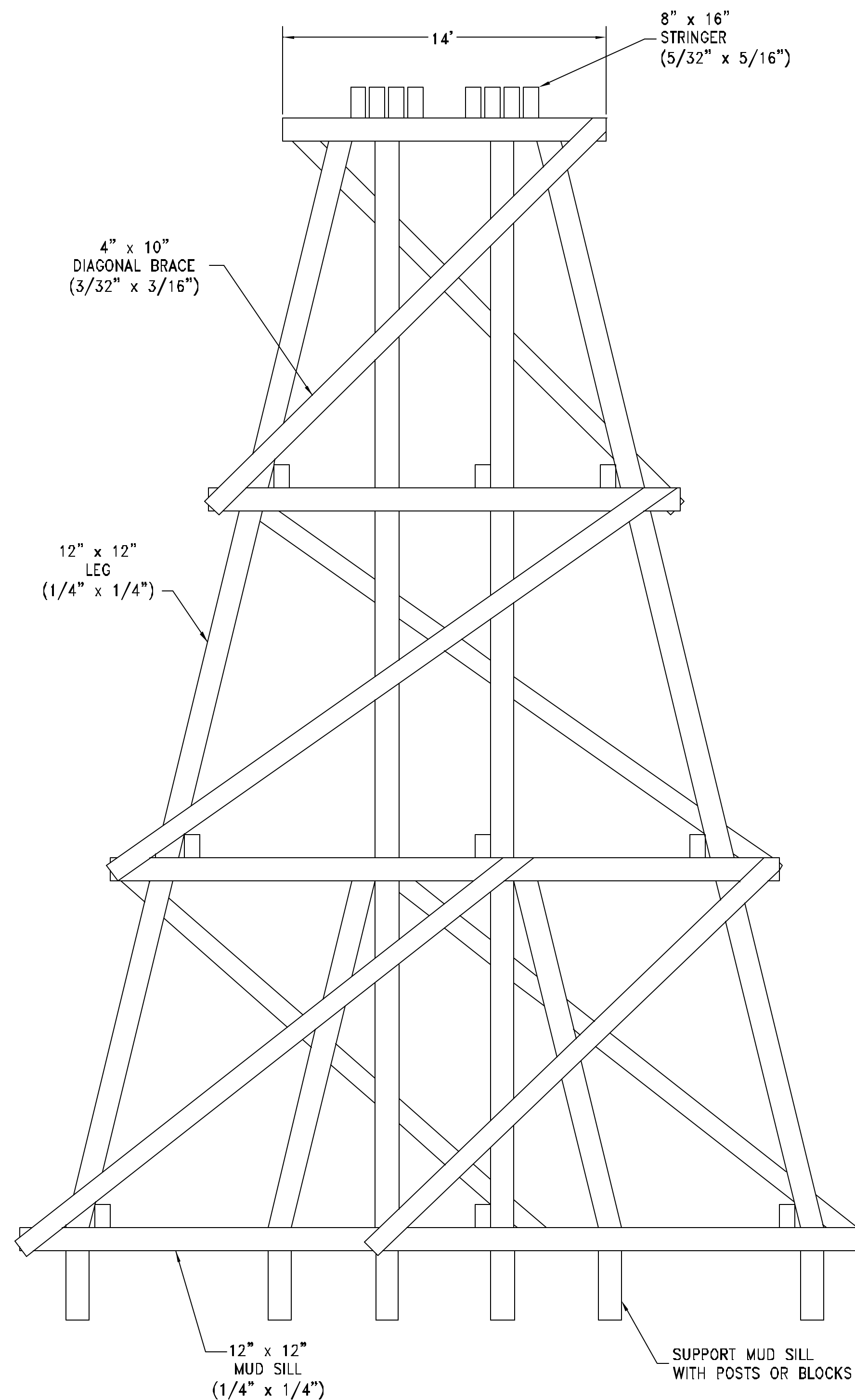
TRUE FRAME BENT or NOTCHED FRAME BENT
