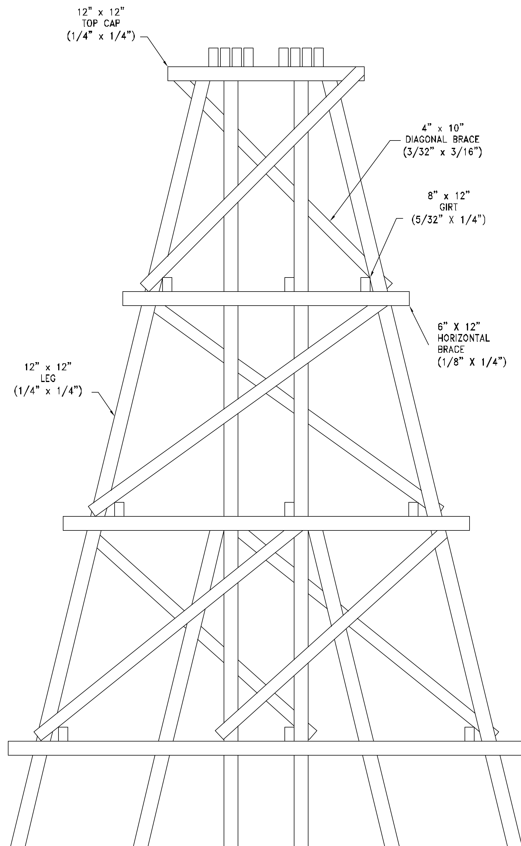
FALSE FRAME TRESTLE BENT
